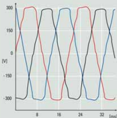
Measurements show clear distortion of the mains voltage as the reaction to non-linear consumers.
