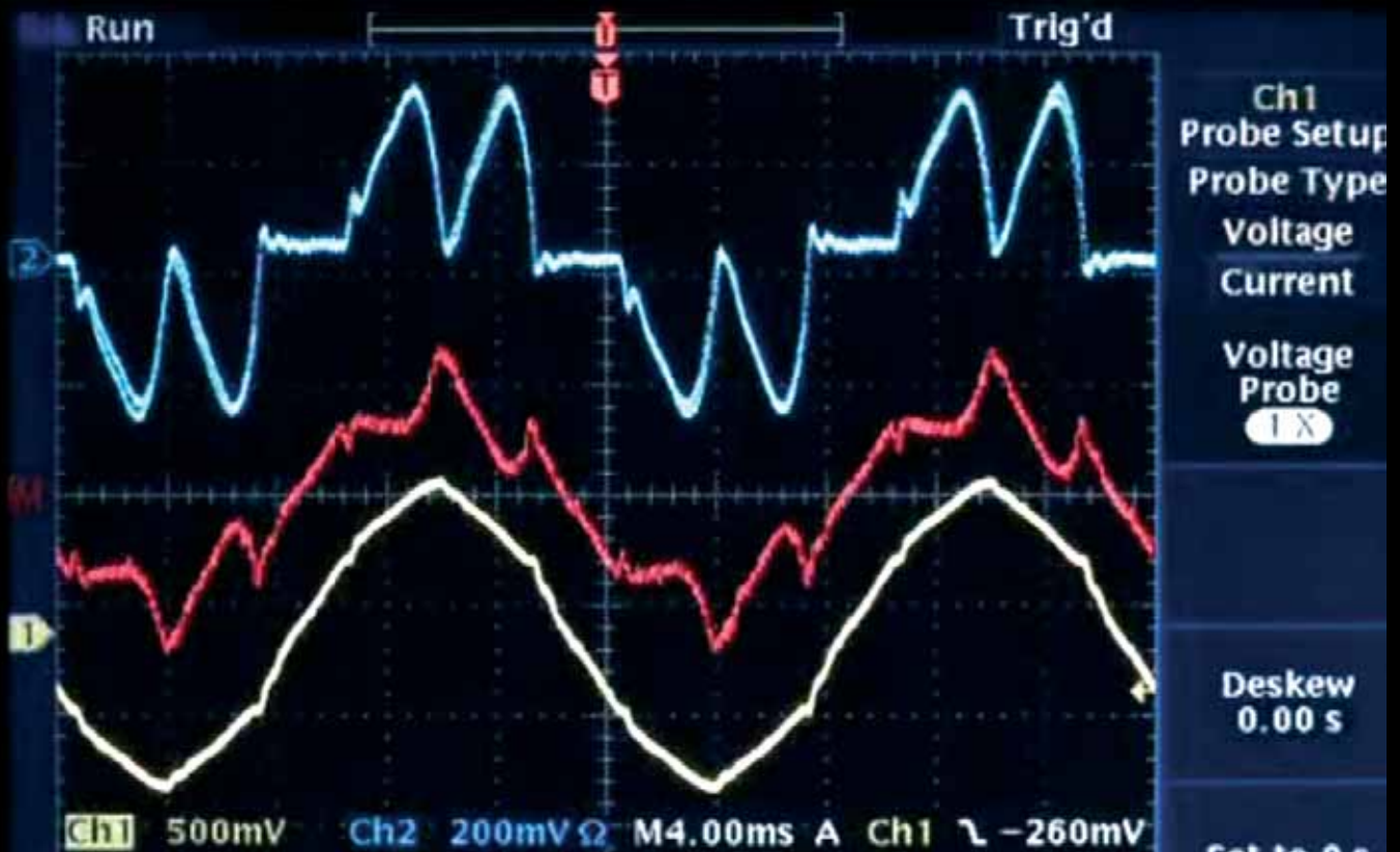
With active filtering the distortion is monitored and analysed. A corrective current is then injected in counter phase to eliminate the distortion.
