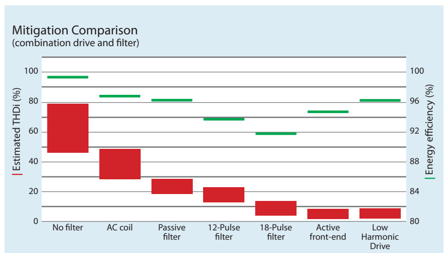
A comparison between different harmonic mitigation principles shows that low harmonic distortion is followed by low energy efficiency – except for active filtering, where the efficiency is relatively good.
