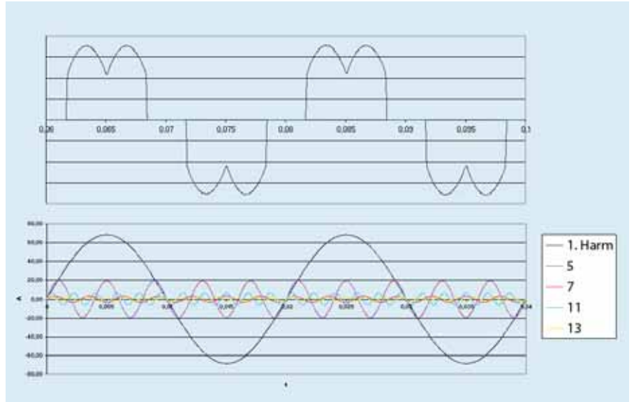
Any periodic function can be described as the sum of a series of sine-wave functions (called a "Fourier transformation") The figure shows the current drawn by a typical drive with dc coils. Underneath it is deconstructed into pure sinus curves. All but the blue curve represents distortion – unwanted and often harmful currents.
